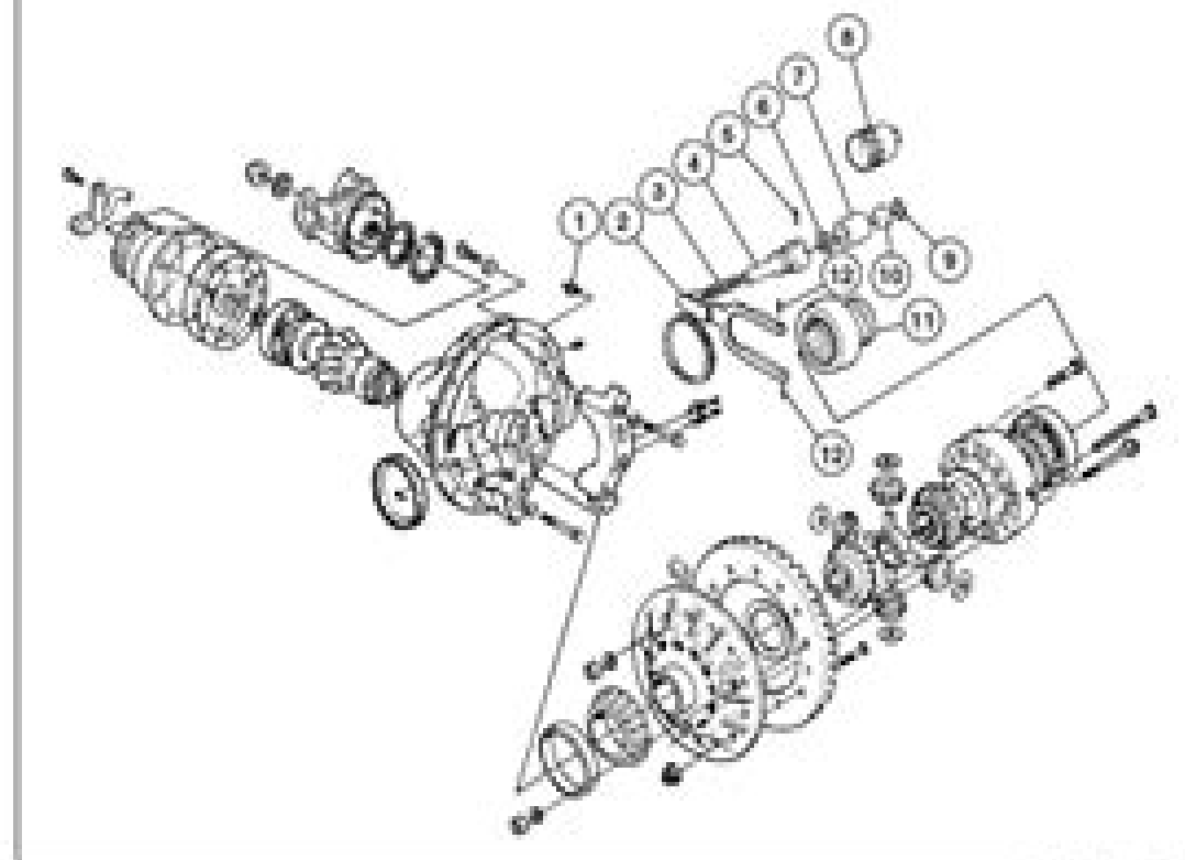
Differential lock assembly
