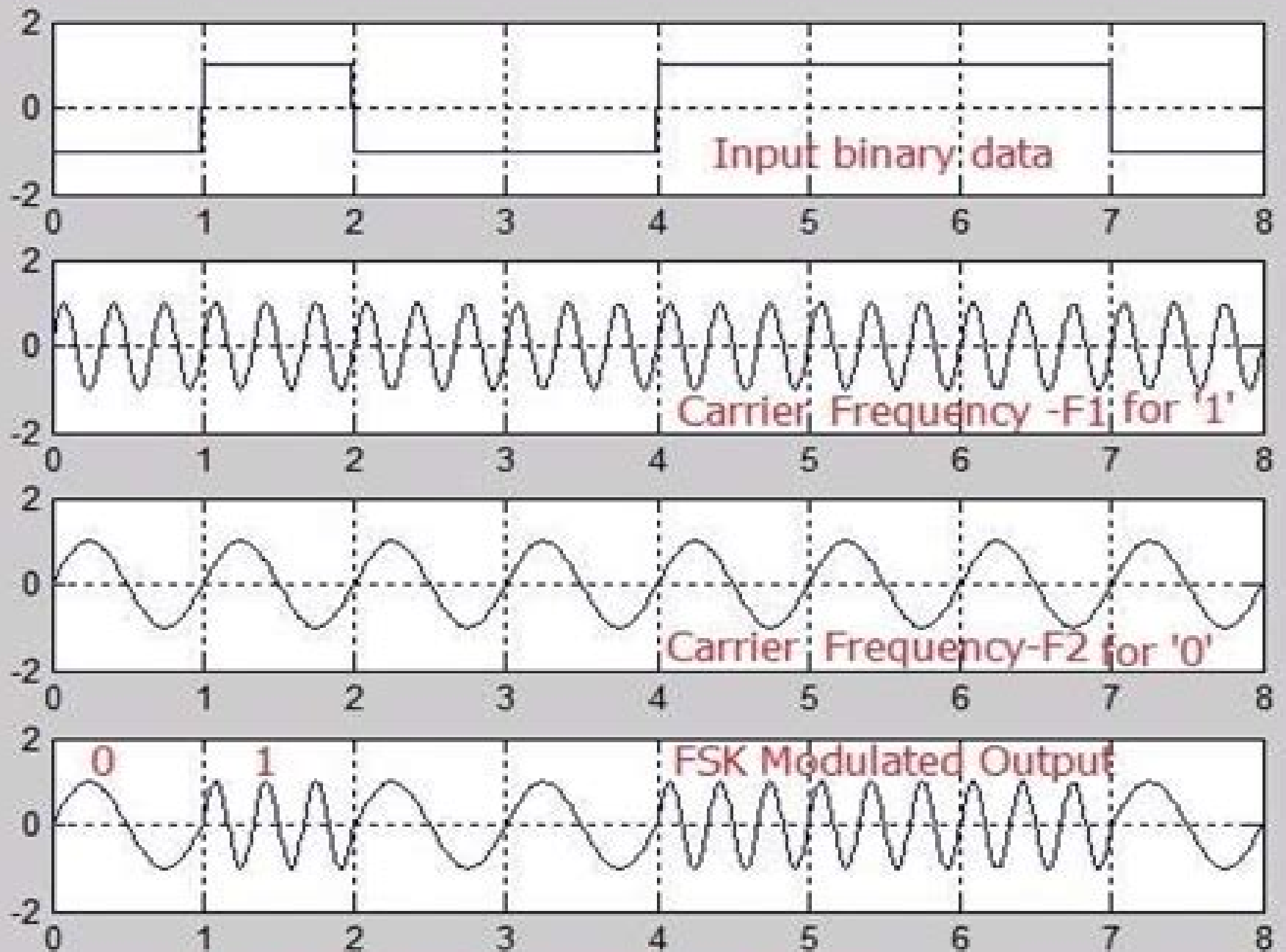
FSK Modulation output waveforms
