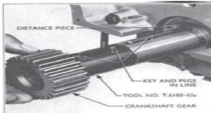
Fig. 15 Fitting the Crankshaft Gear to the Alignment Adaptor
