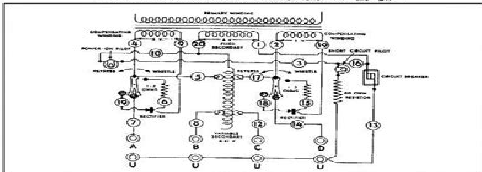
SCHEMATIC WIRING DIAGRAM OF TRANSFORMERS "VW" and "ZW"
