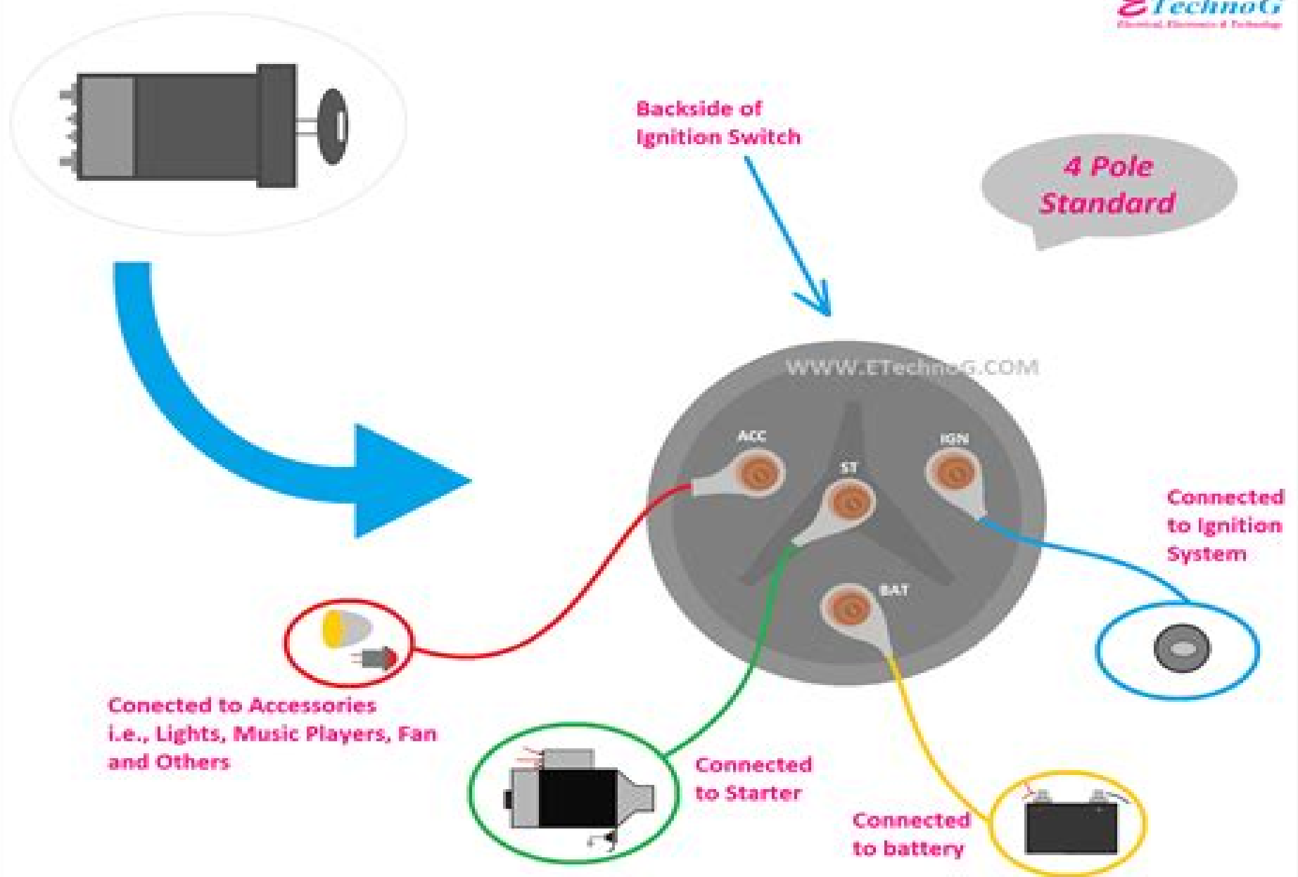
Ignition Switch Wiring Diagram and Connection Guid
