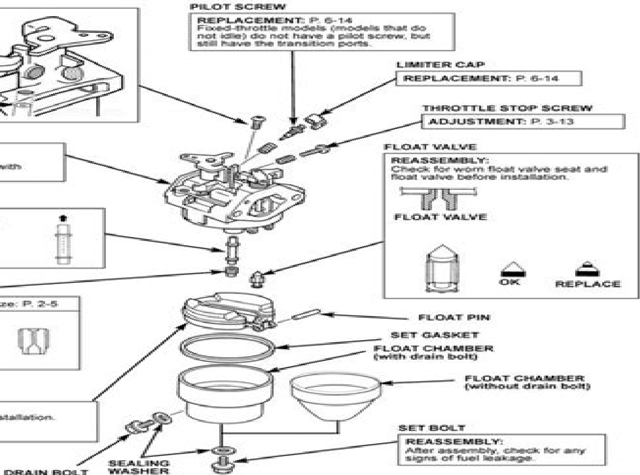
DRAIN BOLT
