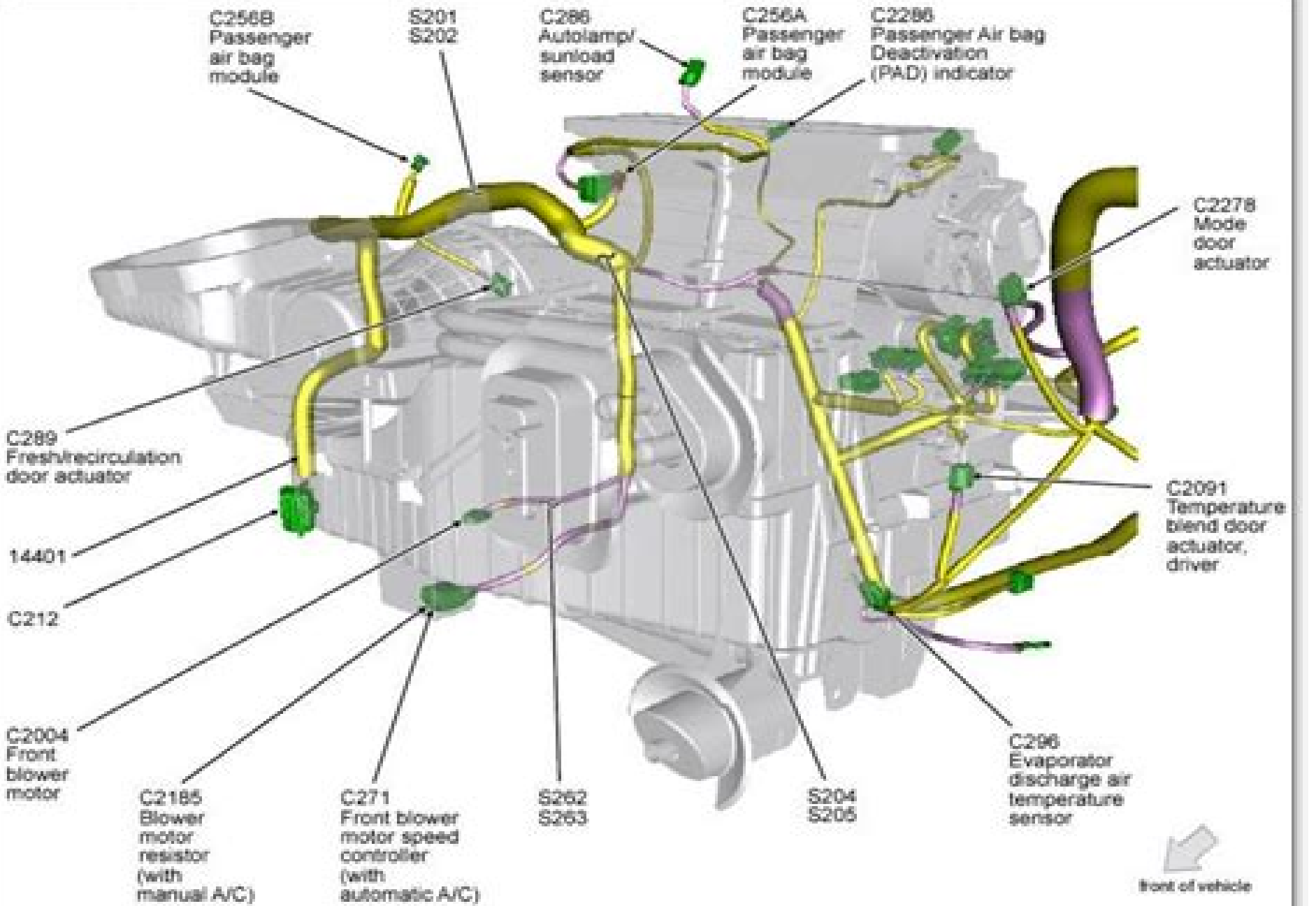
Fig 2: HVAC Unit
