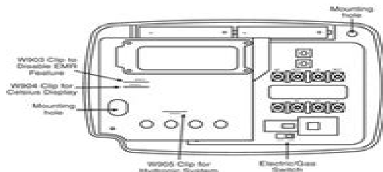
Figure 1. Thermostat base
