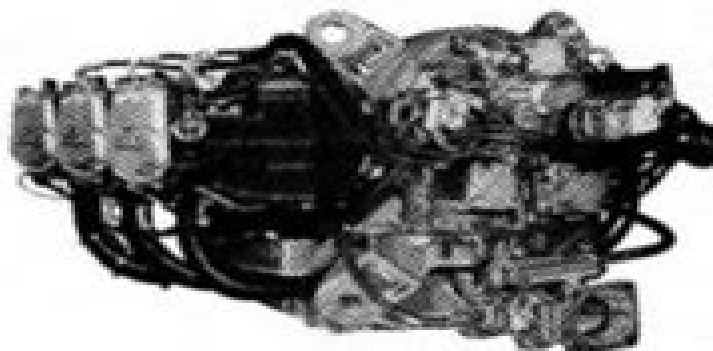
Figure 1-2. Left Rear View IO-540-B1A5
