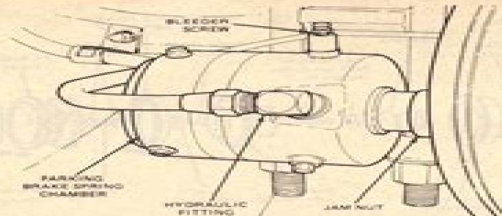
Fig. 39 Parking brake chamber installation
