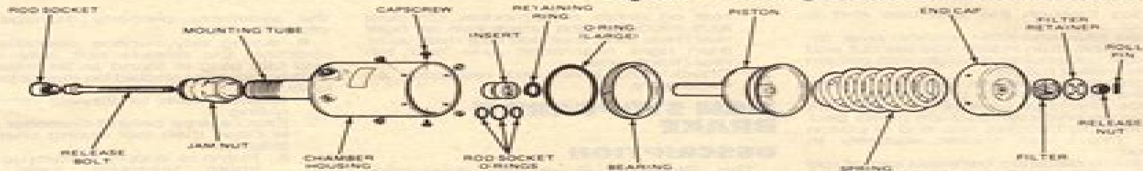
Fig. 40 Exploded view of parking brake chambers. Ford
