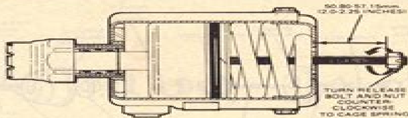
Fig. 38 Caging spring brake unit
