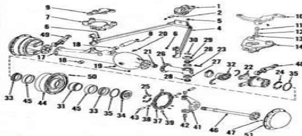
Fig. 9—Exploded view of the front drive axle used when tractors are equipped with "All Wheel Drive". Note items 10 through 14 which are used on International tractors and differ from items 7 and 9 which are used on Farmall tractors.
