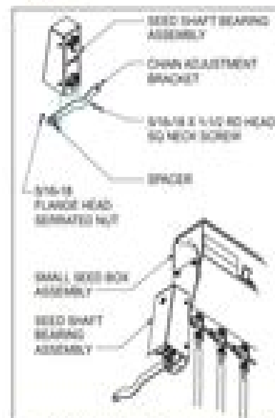
Figure 2-6: Attaching Chain Adjustment Bracket to Small Seed Bearing Assembly
