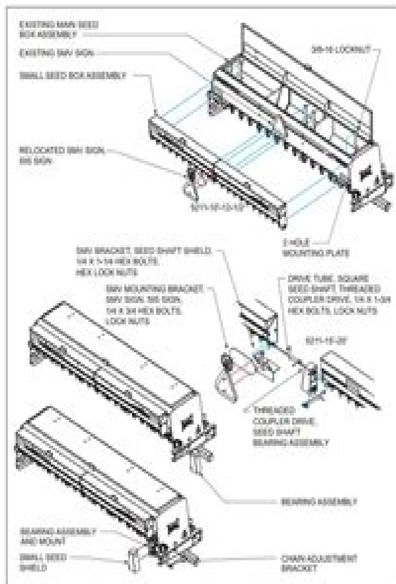
Figure 2-6: Small Seed Assembly Overview (10-12' Drill Shown)
