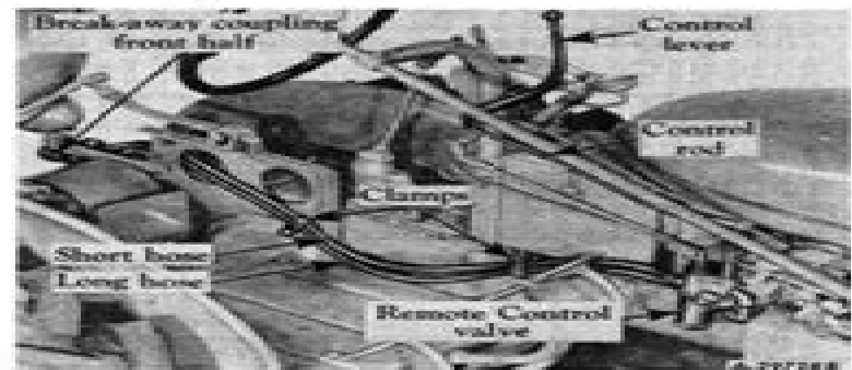
Illustr. 93 Control valve hoses and control lever.
