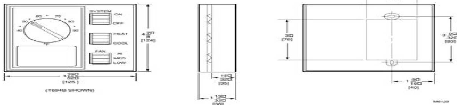
Fig. 2—T694A,B,D,F mounting dimensions in in. [mm].
