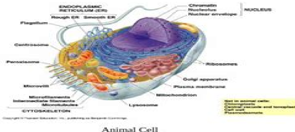
Animal Cell
