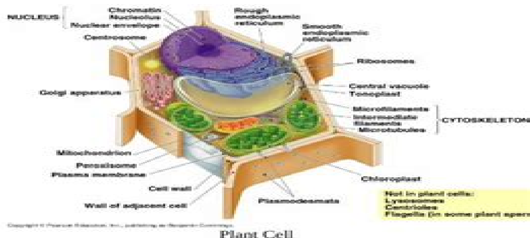
Plant Cell
