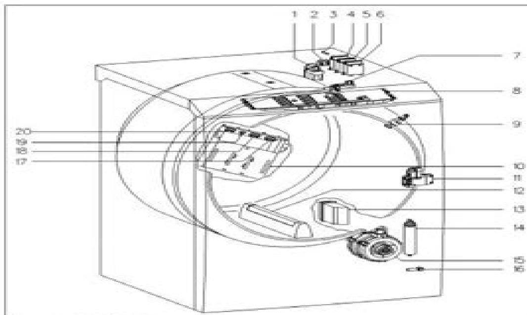
Figure D-1: T 980x Component Layout
