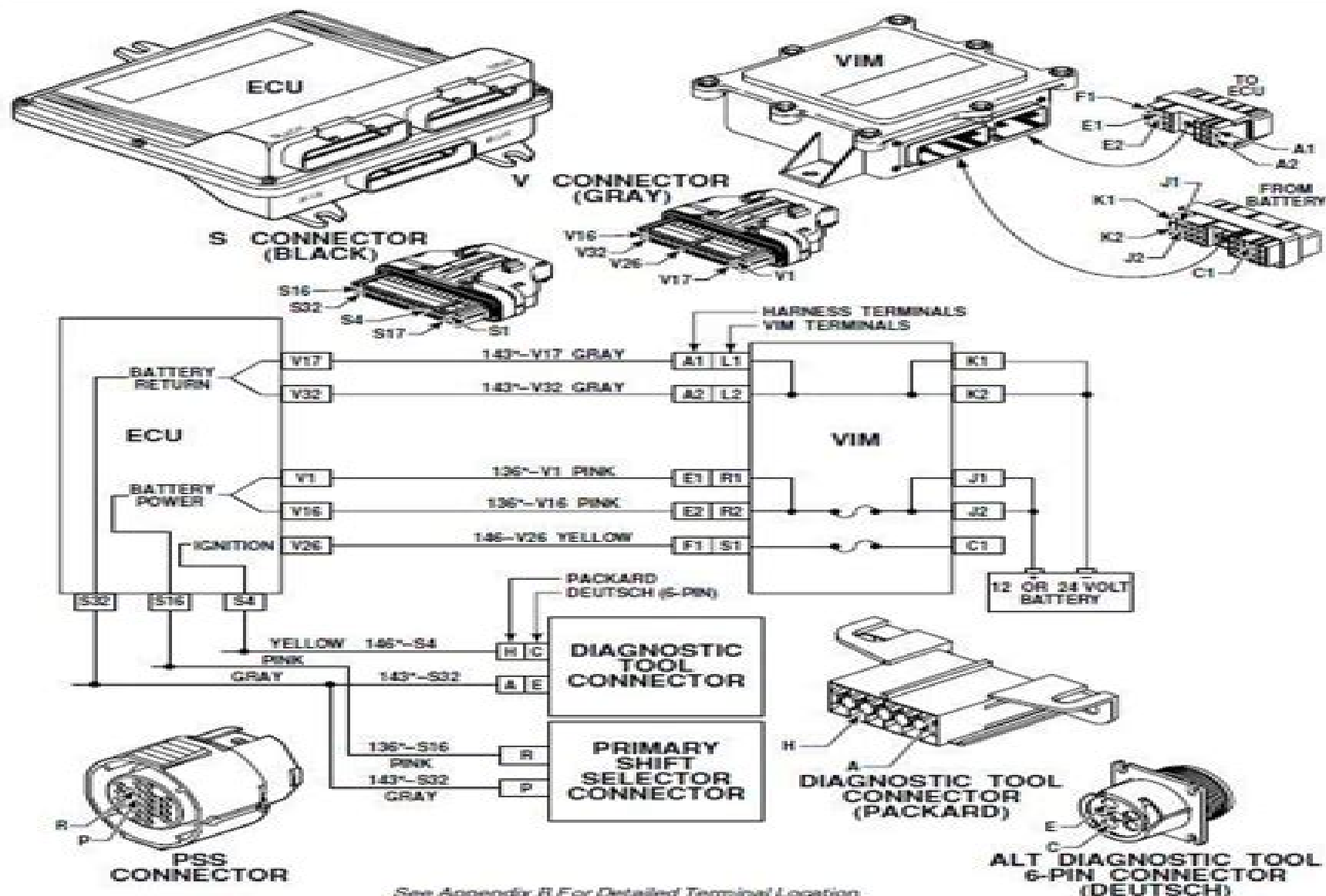
Figure 5-1. Code 13 Schematic Drawing
