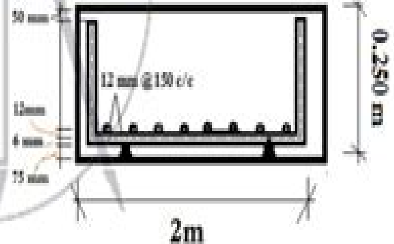
x-Section AA
