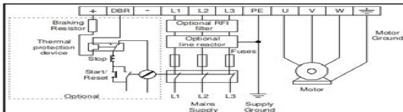
Figure 5.2 Commander SE Size 2 to 4 power terminal connections
