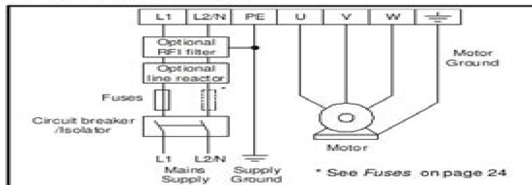
Figure 5.1 Commander SE Size 1 power terminal connections
