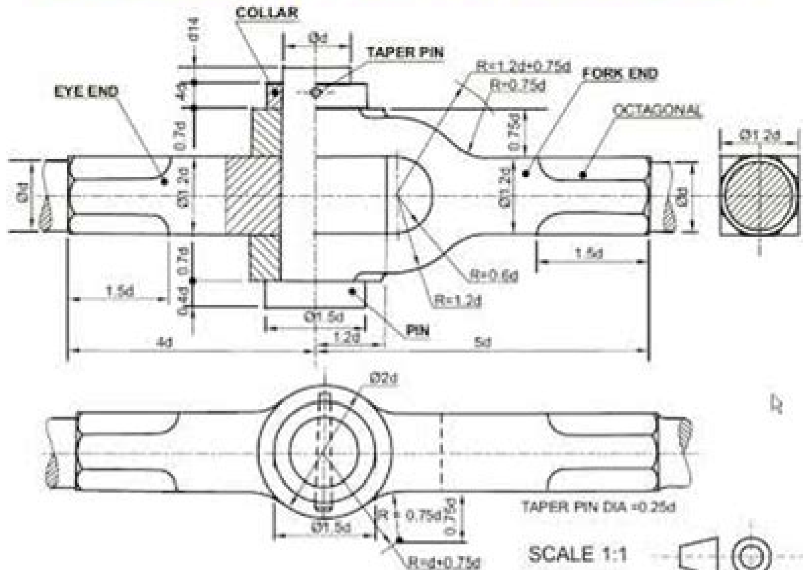
KNUCKLE JOINT
