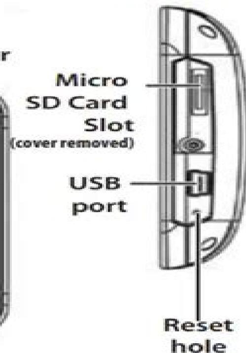
Side panel
