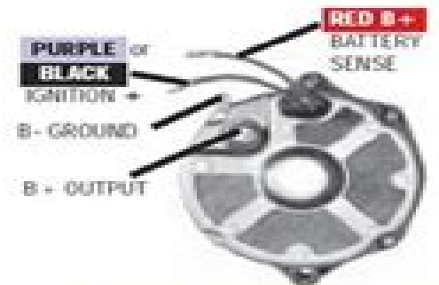
DELCO STYLE FITS MERCURISER & OMC
