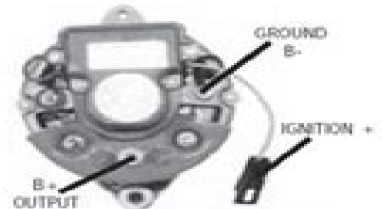
EARLY MOTOROLA STYLE FITS WESTERBEKE AND OTHERS
