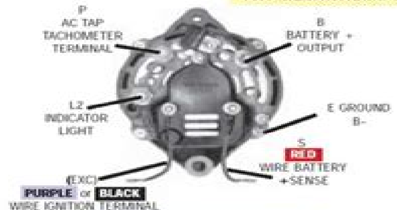
LATE MANDO STYLE FITS MERCURISER AND OTHERS
