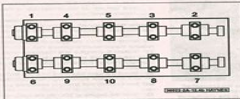
9.7b Loosen the camshaft bearing cap bolts, in several steps, in the sequence shown (2006 and later models)
