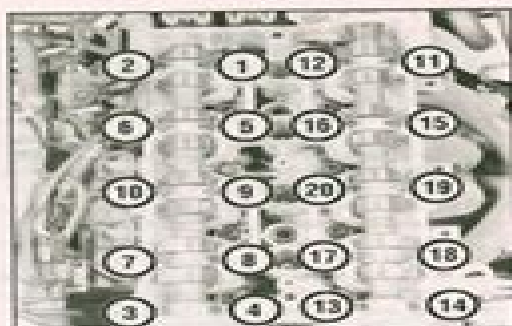
9.7a Loosen the camshaft bearing cap bolts, in several steps, in the sequence shown (2005 and earlier models)
