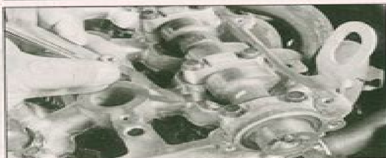
9.3 Measure the lifter-to-cam lobe clearance with a feeler gauge
