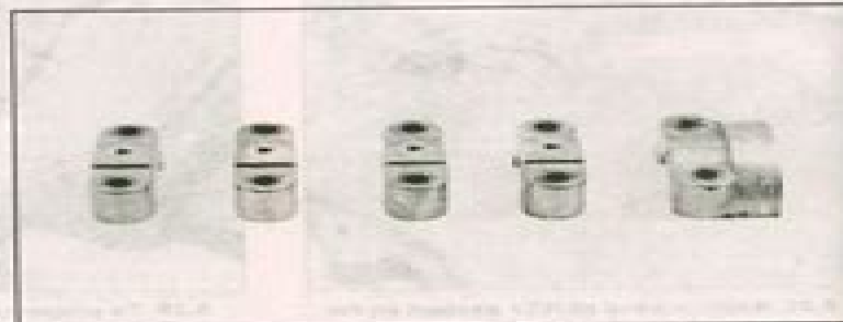
9.7c All cam bearing caps are marked I for intake or E for exhaust; the front cam bearing caps can be identified by their shapes; the others are numbered from front to rear of the engine and have arrowhead marks that point to the front
