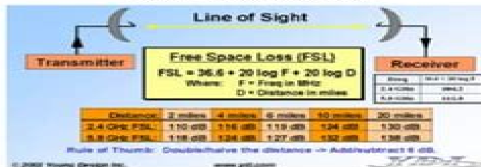
Figure 1 – Free Space Loss (FSL)
