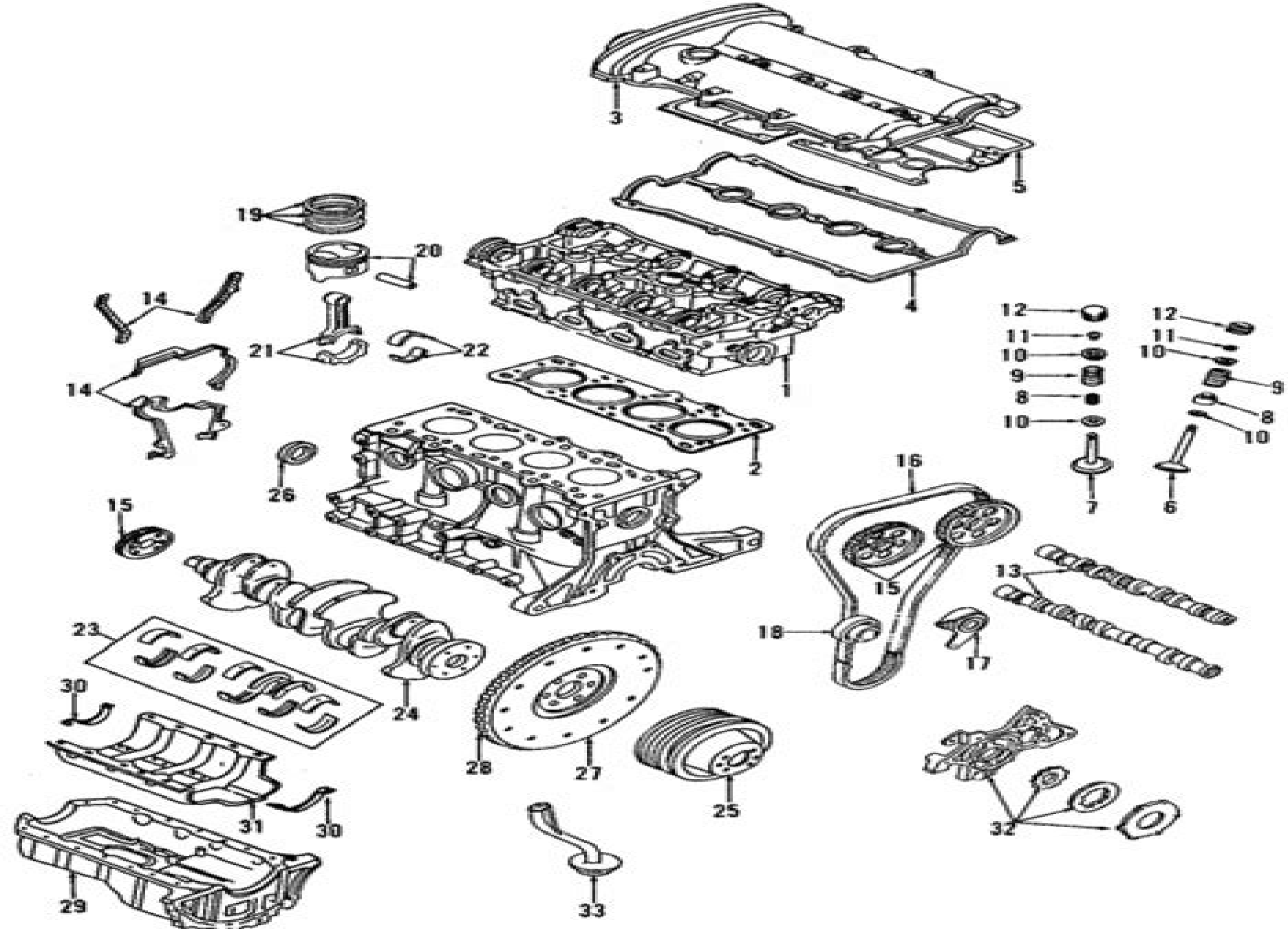
ENGINE-4 CYLINDER, MIATA MX5
