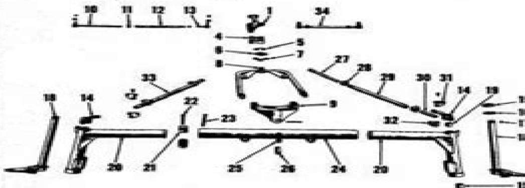
Fig. 6-Exploded view of adjustable wide front axle used on Farmall "Hi-Clear" models. Note the auxiliary stay rod assemblies.
