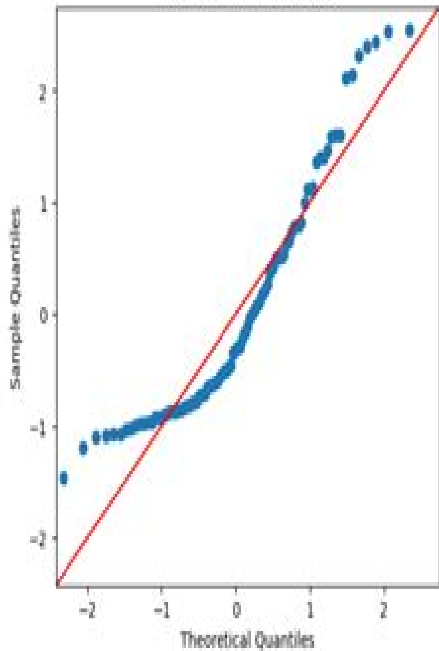
Non-Normal Residuals
