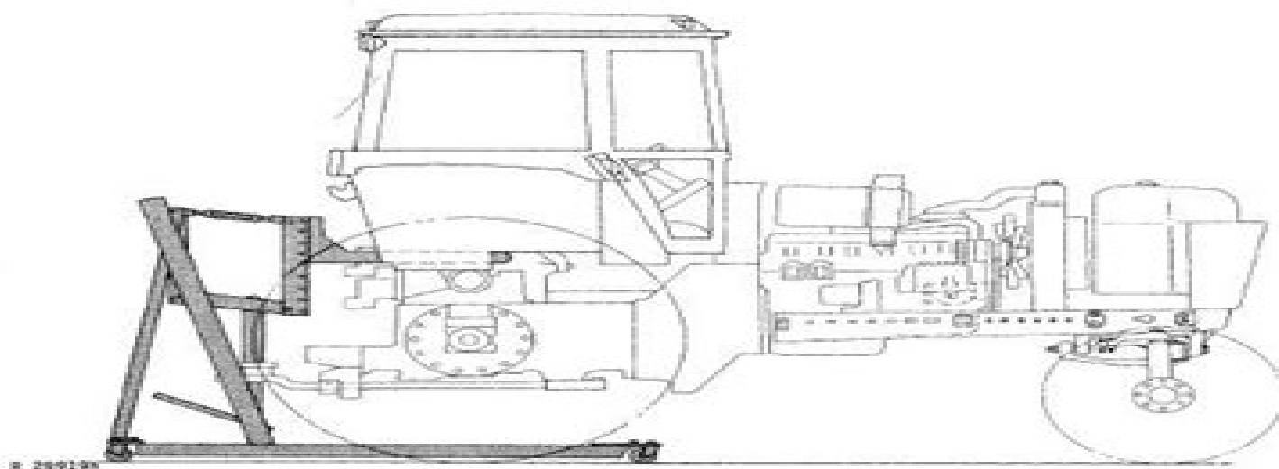
Fig. 12-Removing Sound-Gard Body With Control Support
