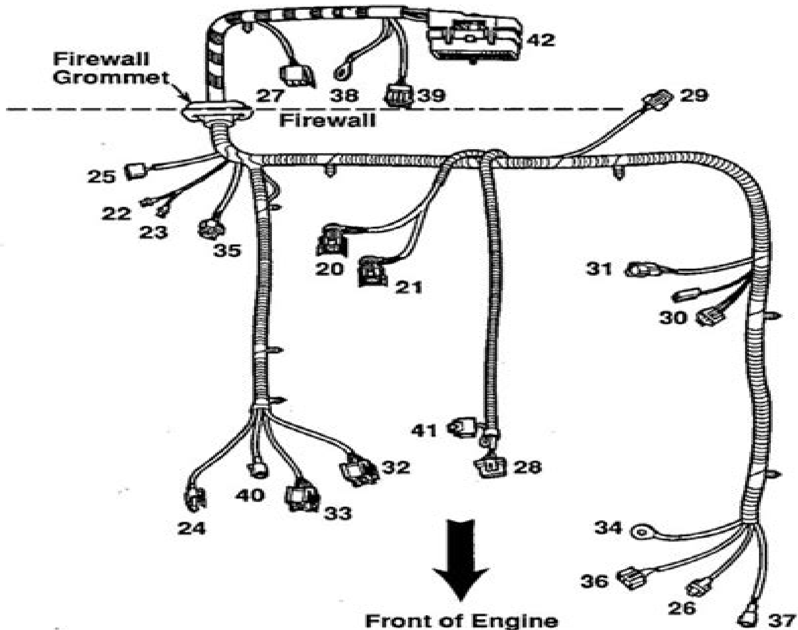
Figure 2 MAIN HARNESS M-12071-C302
