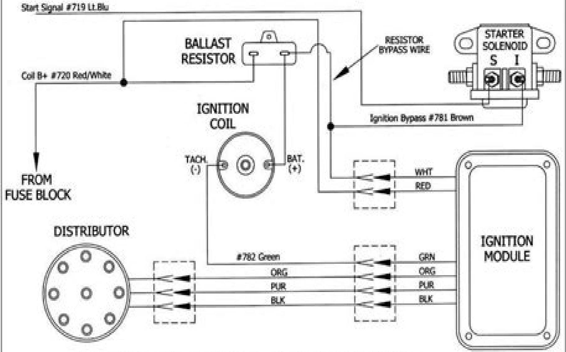
Illustration E Duraspark Electronic Ignition (Start/Run) System
