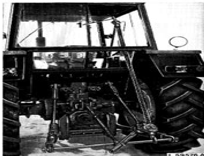
Fig. 15 — Connecting Hand Winch
