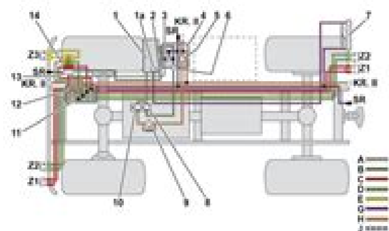
Hydraulic diagram of work hydraulics (front and rear work hydraulic system)
