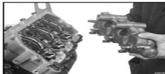
Figure 252 Align oil rail assembly to injector oil inlets
