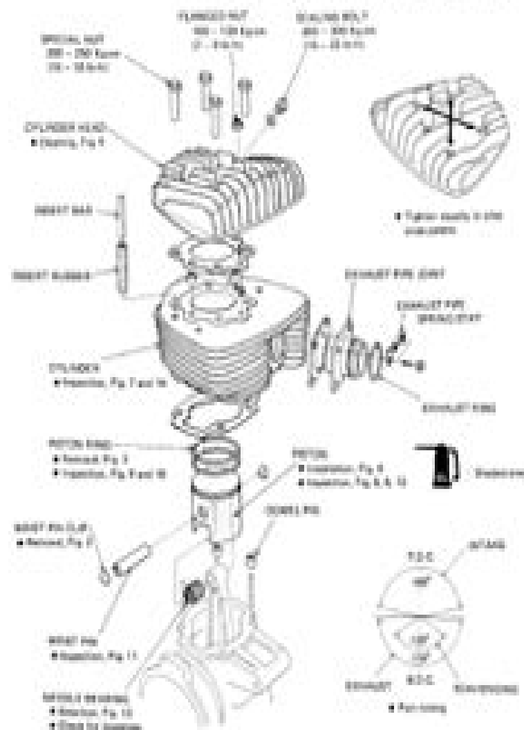
Fig. 1. Cylinder/Piston (Separately Assembly)
