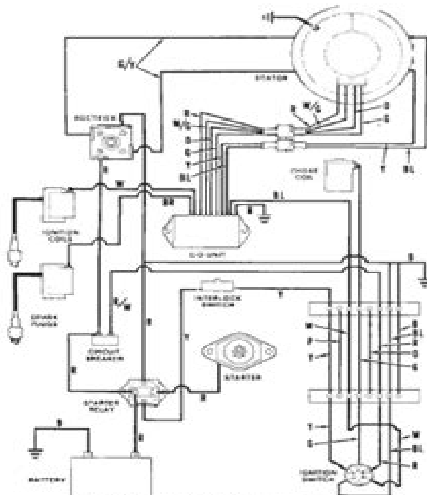
Fig. P2-9—Wiring schematic of Magnaspark ignition system.
