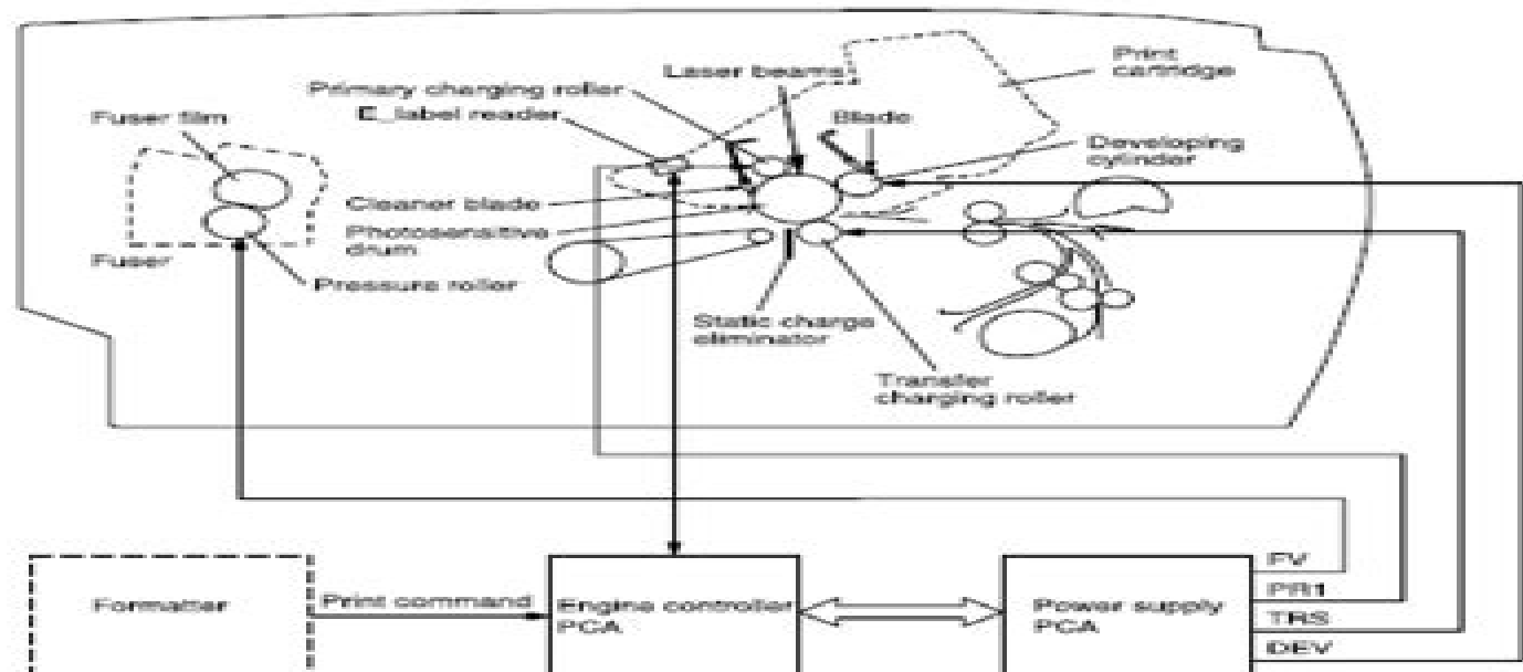
Figure 18. Image-formation system
