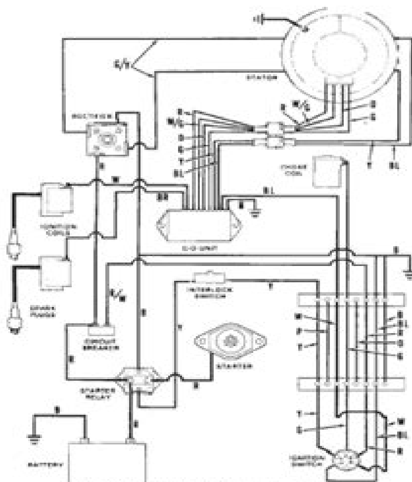
Fig. P5-9—Wiring schematic of Magnapower ignition system.
