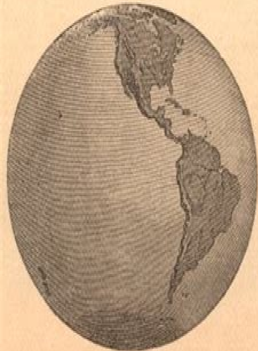
WESTERN HEMISPHERE.
