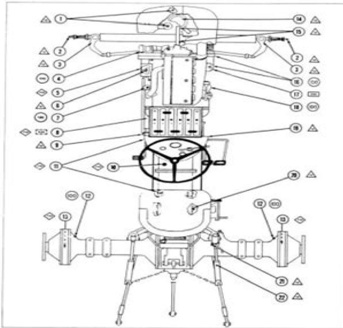
Fig. 1 - Lubrication Chart (Descent Stage)
