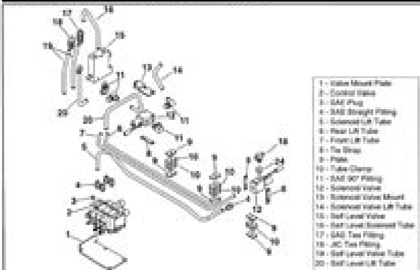
Fig. 9-29 Exploded view of LiFTit Self-Leveling Hydraulics - Chassis - SX Models
