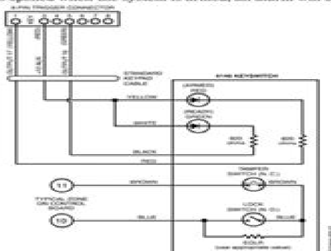
Figure 12. Keyswitch Wiring Connections
