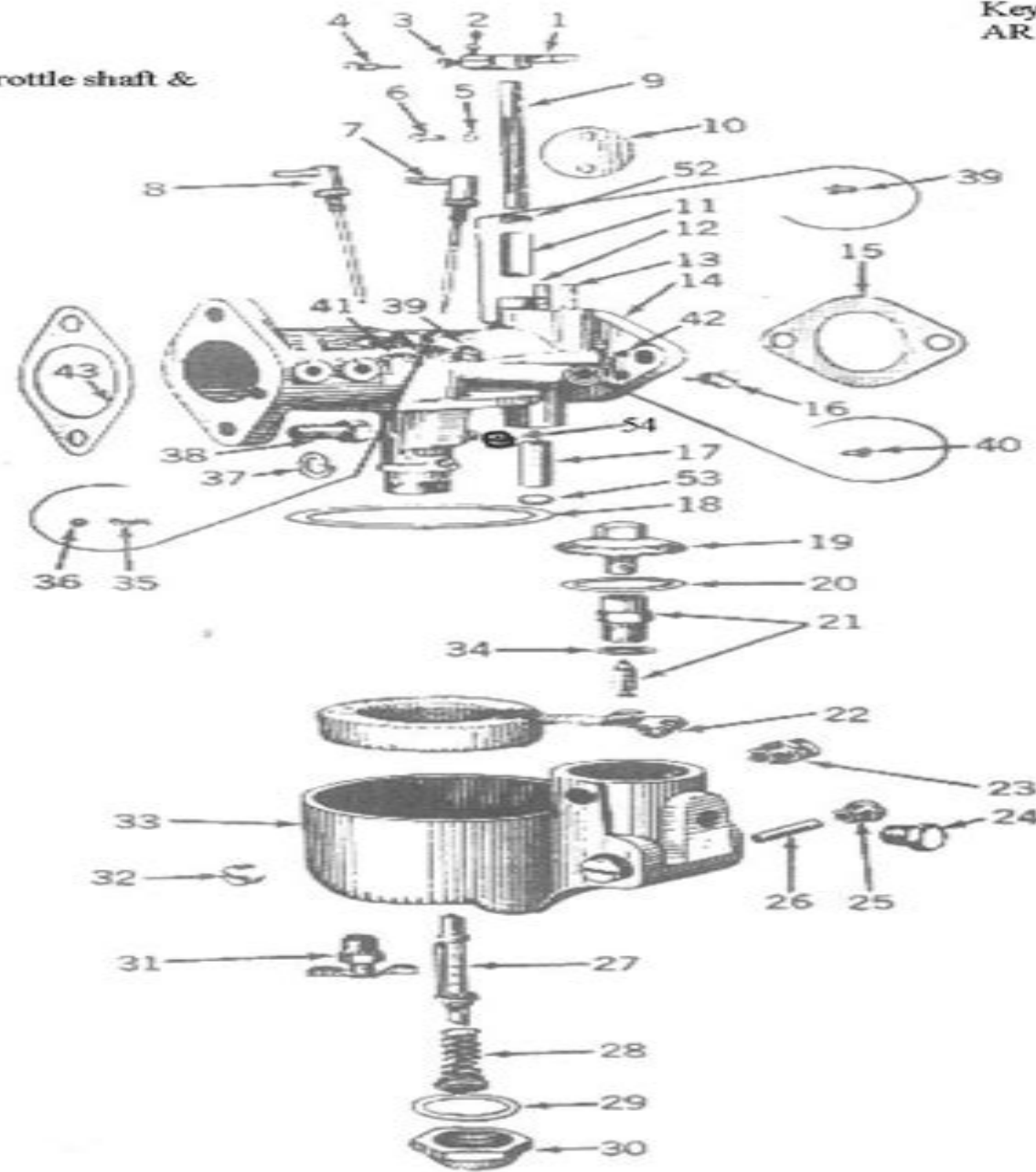
Key 1B AR10024 throttle arm
