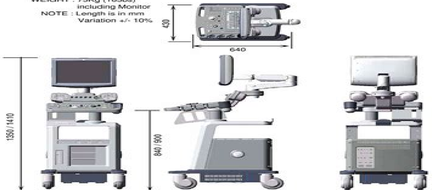
Figure 3-13 Overall Dimensions
