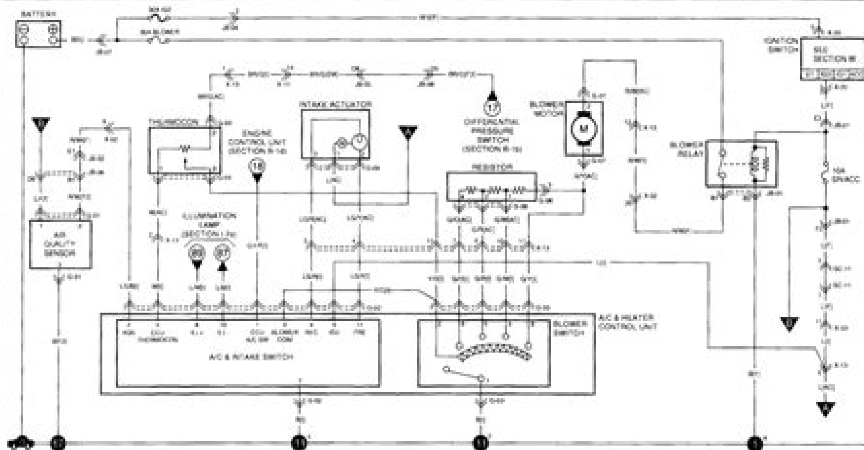
G-01 AIR QUALITY SENSOR (P/S)
