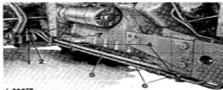
Fig. 2 — Disconnecting Hydraulic Lines
