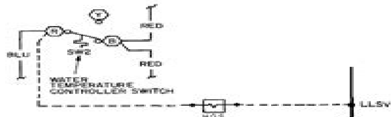
Fig. 8 — Hot Gas Bypass Field Wiring; 30GT Units
