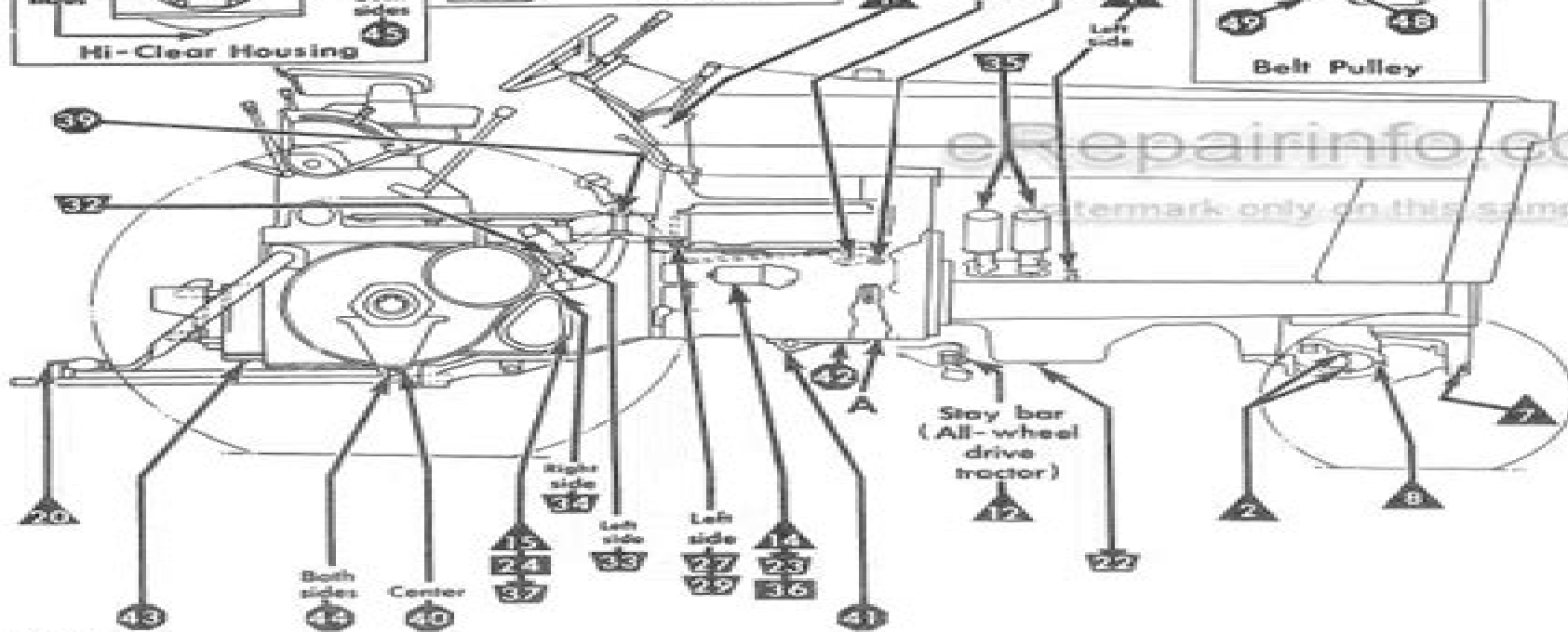
Right side view of tractor.
