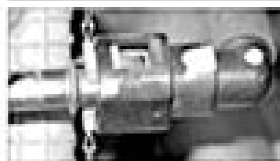
13 13a The fuel pump fitting, remove both sides with your fingers, then pull the fuel pipe and the fitting apart
