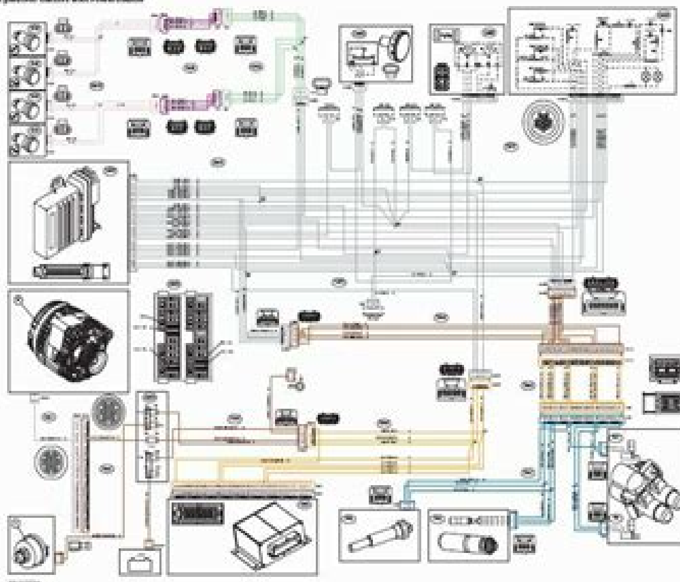
Electronic linkage on platform trolleys with PowerBus®
