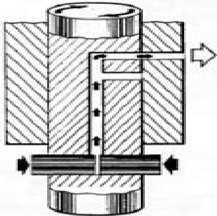
FIG. 113a WORKING PRINCIPLE OF D.P.A. PUMP
